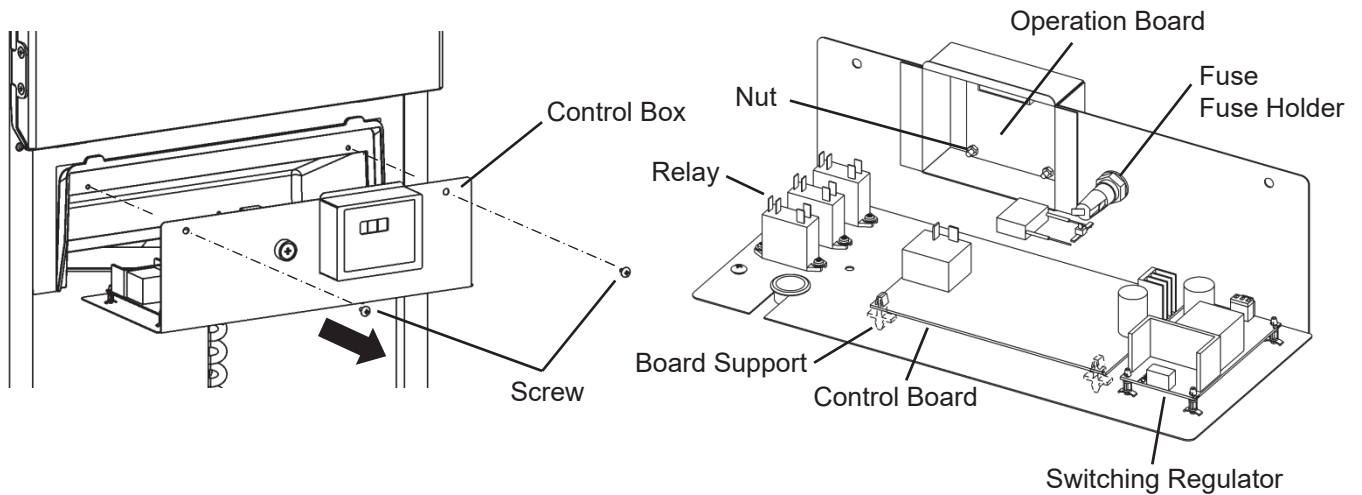
Control Box
