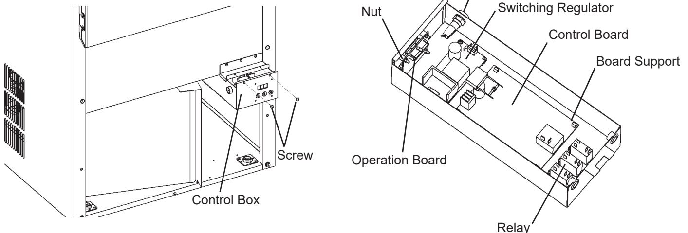
Control Box
